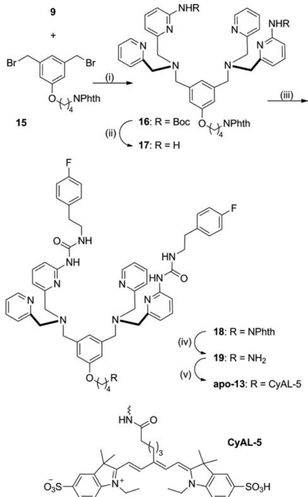
Scheme 4. Synthesis of Modified Fluorescent Probe 13 a
