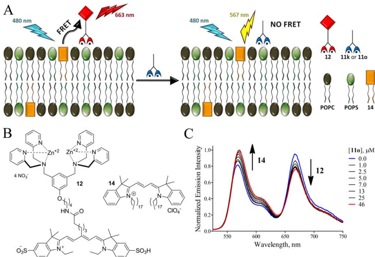
Figure 2. Schematic cartoon of the FRET displacement assay (A). Chemical structures of fluorescence energy acceptor 12 and lipophilic energy donor 14 (B). Emission profile for the FRET displacement experiment using anionic PS-rich vesicles (POPS:POPC: 14 , 50:49:1) and lead candidate 11o (C).
